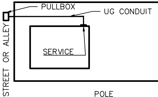
CASE 1: BACKYARD POLE LINE (NEW UG) – BWP INSTALLS CONDUCTOR TO 1ST PULLBOX, CONTRACTOR INSTALLS FROM PULLBOX TO PANEL.
