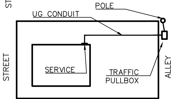
CASE 3: STREET/ALLEY (PULLBOX ADJACENT TO PROPERTY) – BWP INSTALLS CONDUCTOR TO PULLBOX ADJACENT TO PROPERTY, CONTRACTOR INSTALLS FROM PULLBOX TO PANEL. BWP MUST BE ONSITE DURING CONDUIT WORK INSIDE ENERGIZED BOX IF REQUIRED.
