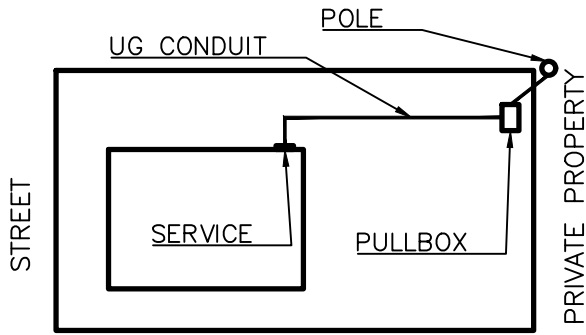
CASE 1: BACKYARD POLE LINE (NEW UG) – BWP INSTALLS CONDUCTOR TO 1ST PULLBOX, CONTRACTOR INSTALLS FROM PULLBOX TO PANEL.
