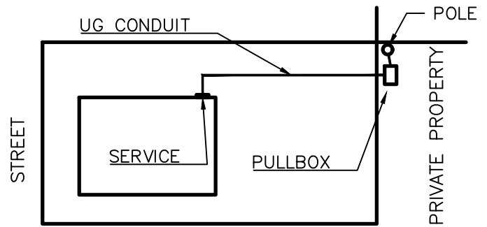
CASE 2: BACKYARD POLE LINE (EXISTING UG) – CONTRACTOR INSTALLS CONDUCTOR FROM PULLBOX TO PANEL, BWP TERMINATES INSIDE PULLBOX. BWP MUST BE ONSITE DURING WORK INSIDE ENERGIZED BOX. CONTRACTOR RESPONSIBLE TO COORDINATE ACCESS TO PULLBOX IF NOT LOCATED ONSITE.
